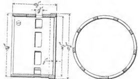
Figs. 2143-2144. Piston Valve Steam Chest Bushing.
